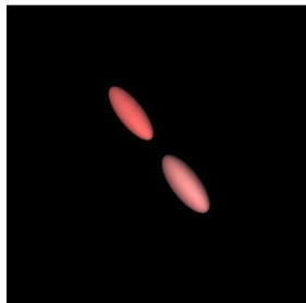
Two ellipsoids.
